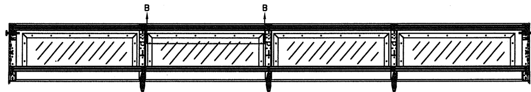
LONG PANEL TOP GLAZED SECTION (STRUT AND STILE LAYOUTS)
